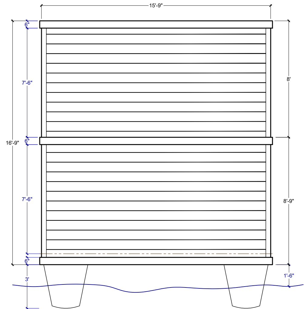
○ STERN ELEVATION
