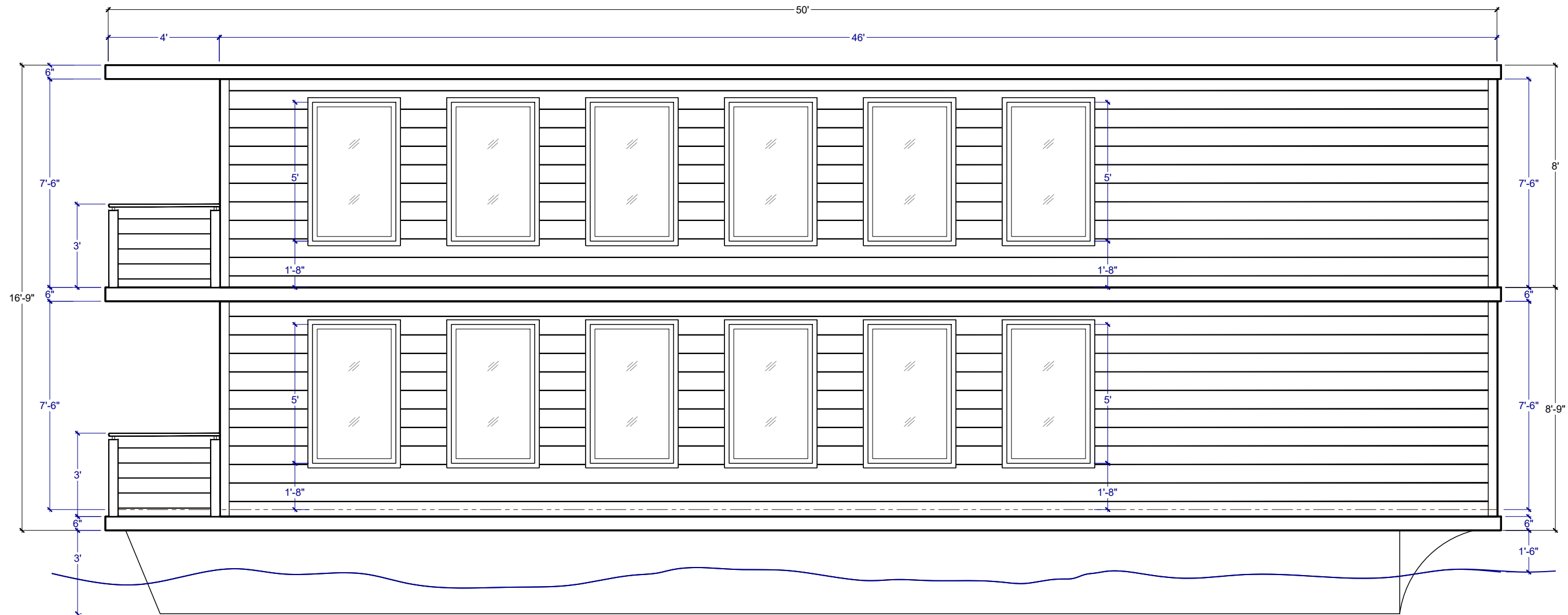
○ STARBOARD ELEVATION
