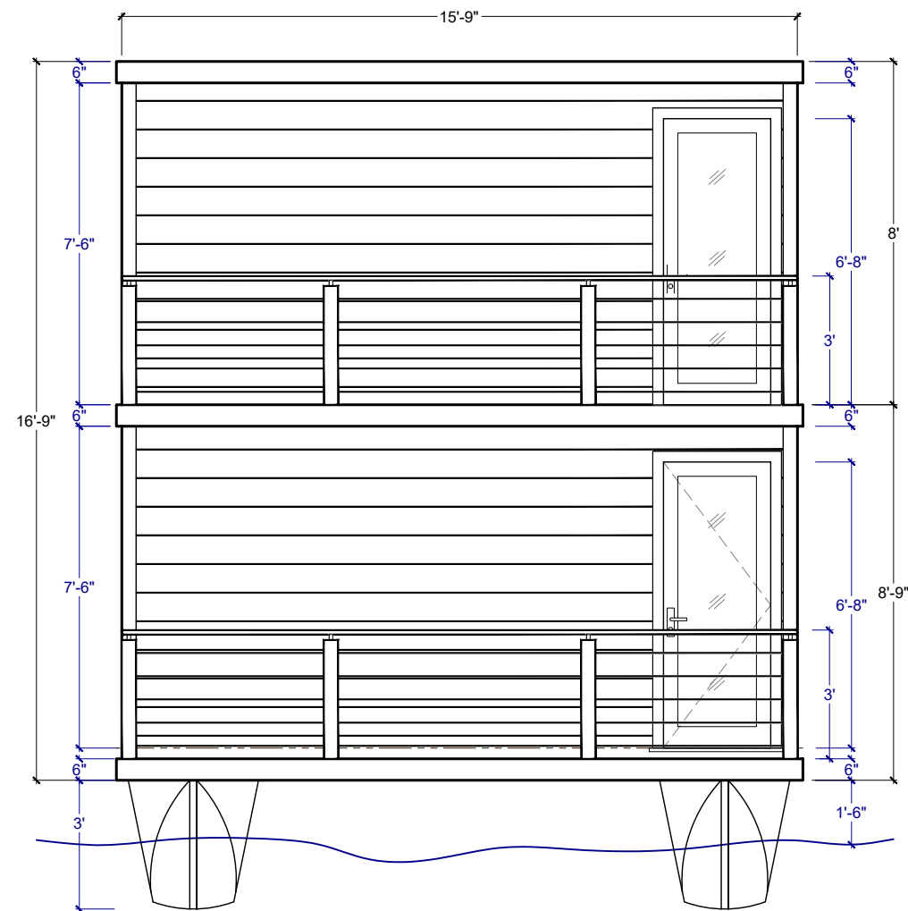
○ BOW ELEVATION
